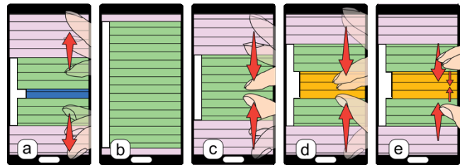
Figure 5: Pinch-and-Flick gestures.
